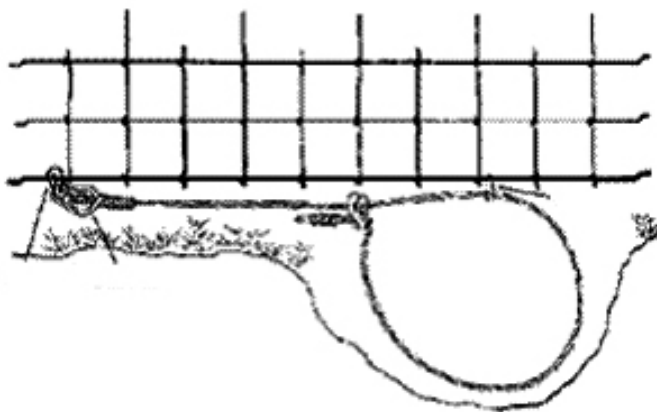
Figure 13-14. A crawl-under cable restraint.
